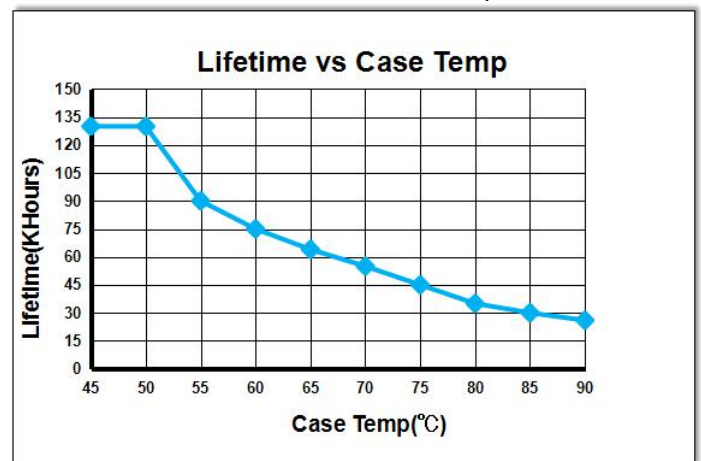
Lifetime VS Case Temp
