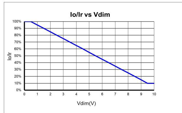
2:Negative logic
