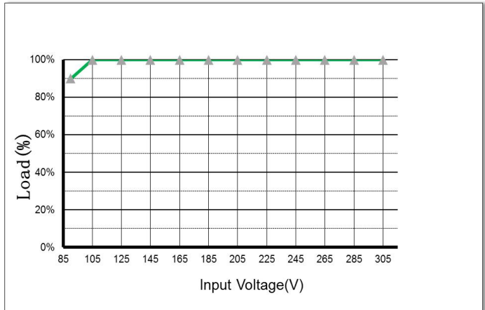
Static Characteristics
