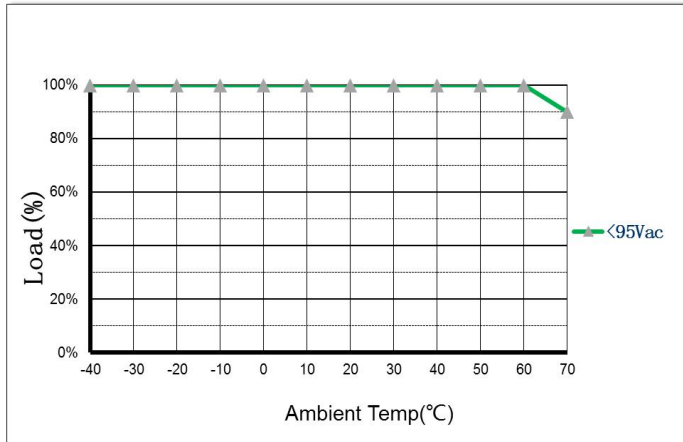
Derating Characteristics
